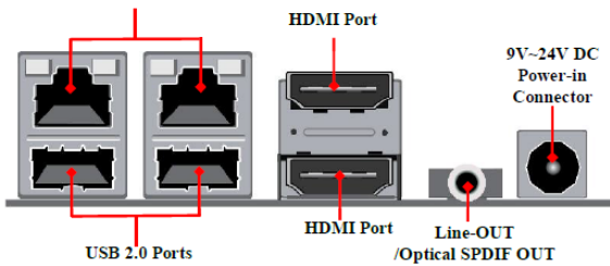
Front IO Panel Diagram:
